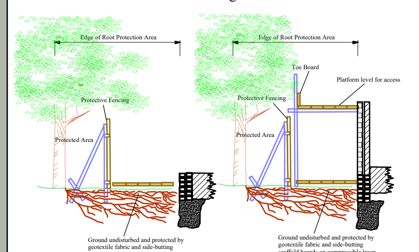
Scaffolding (and Extended Work Space) Within Protection Zones
